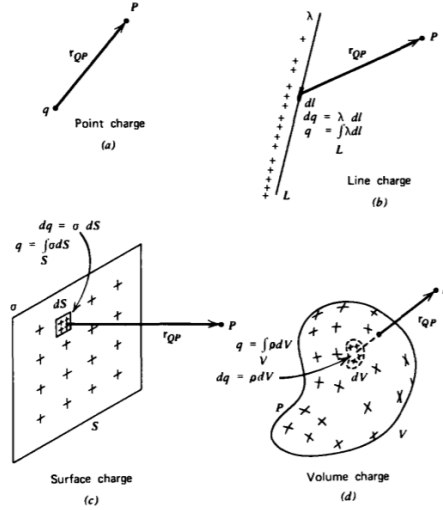
Figure 6: Charge distributions
