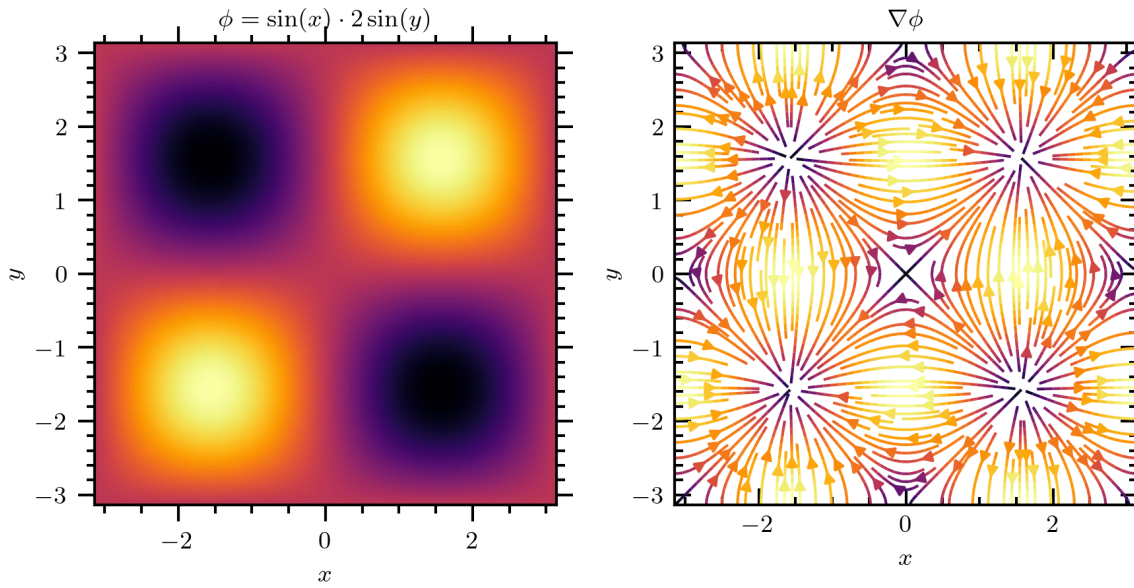
Figure 2: A scalar field and its gradient
